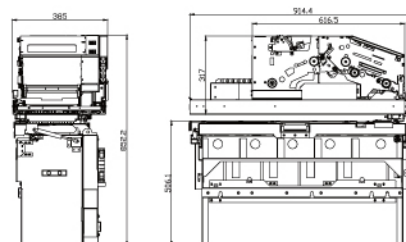
Rear Service
