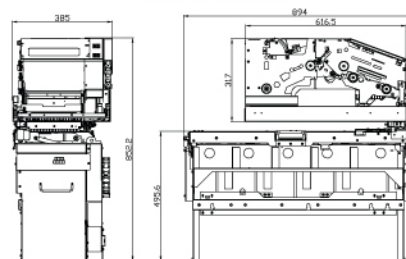
Front Service
